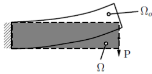
Inverse motion form finding problem
